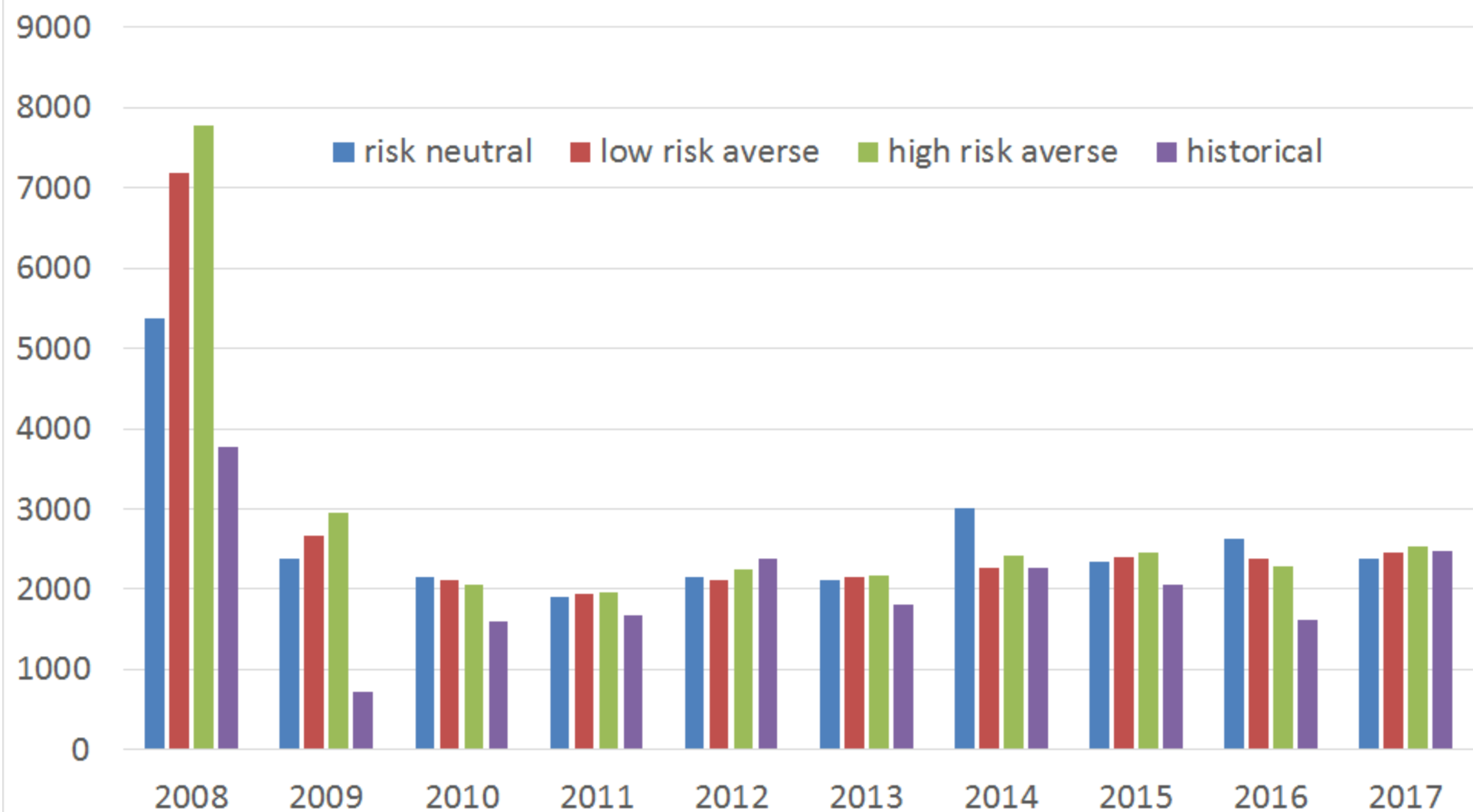
Simulated Ricardian rents ($M) assuming high gas cost
